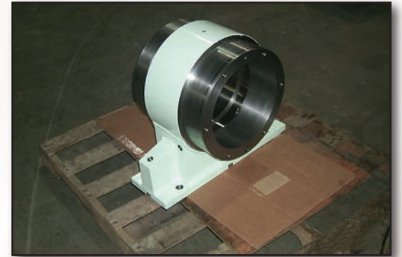
MMW designed / built 340mm bore bearing housing for paper machine
