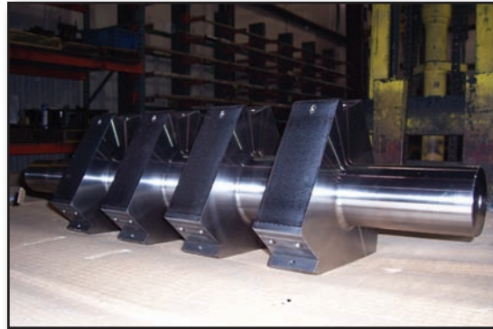
MMW reverse engineered and machined from a solid workpiece for recycled plastics shredder
