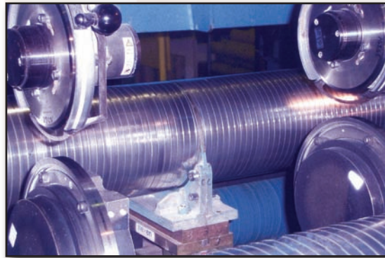
In-place machining on paper winder slitter roll
